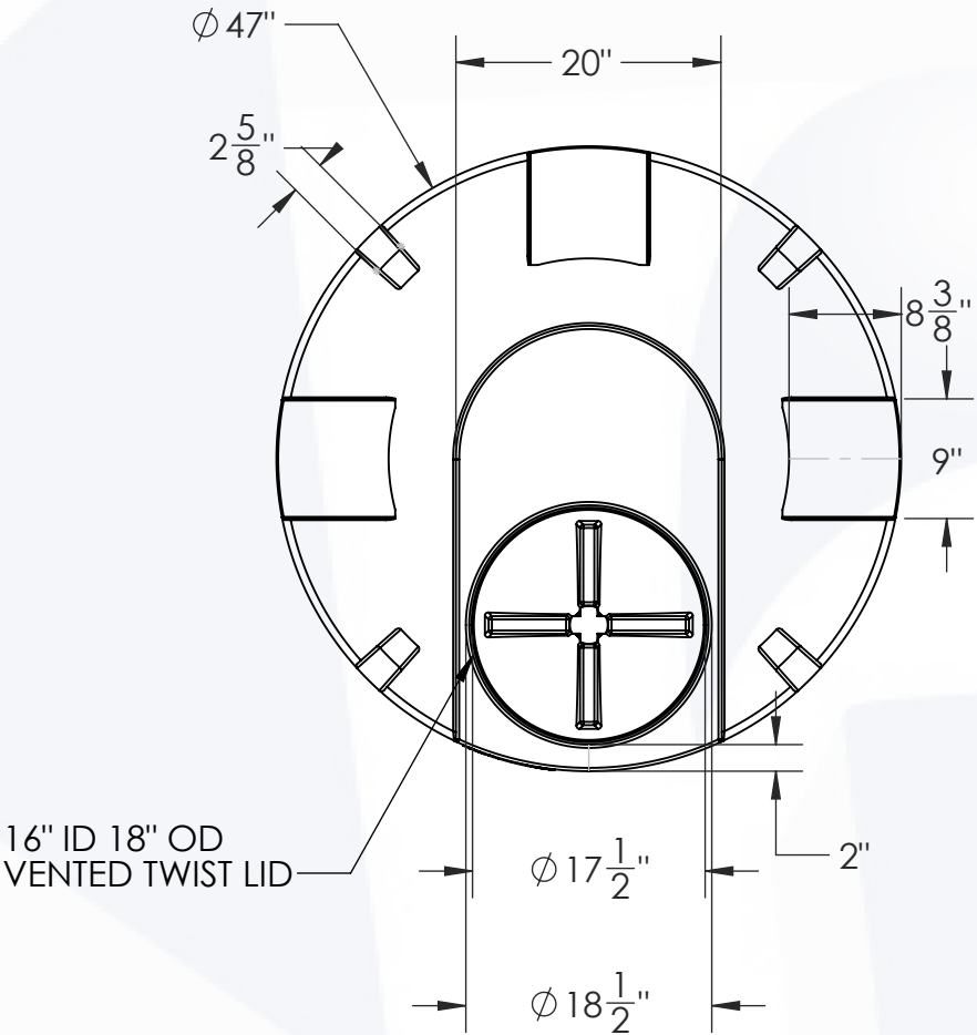
PLAN VIEW
