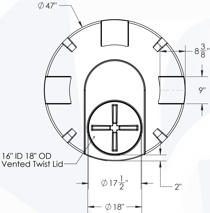
PLAN VIEW
