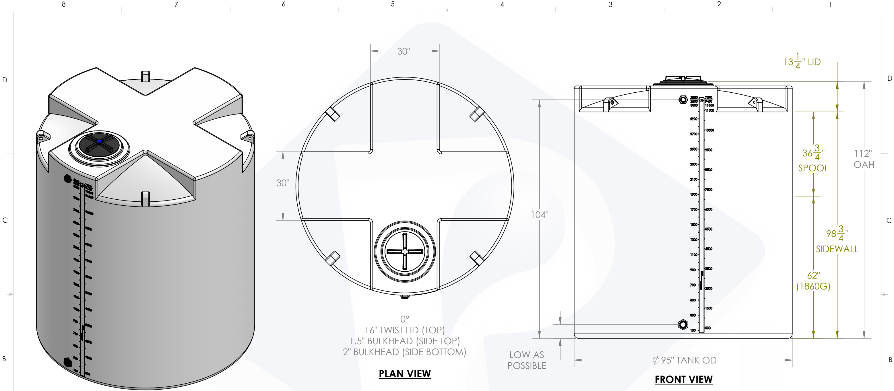
ISOMETRIC VIEW (FRONT)
