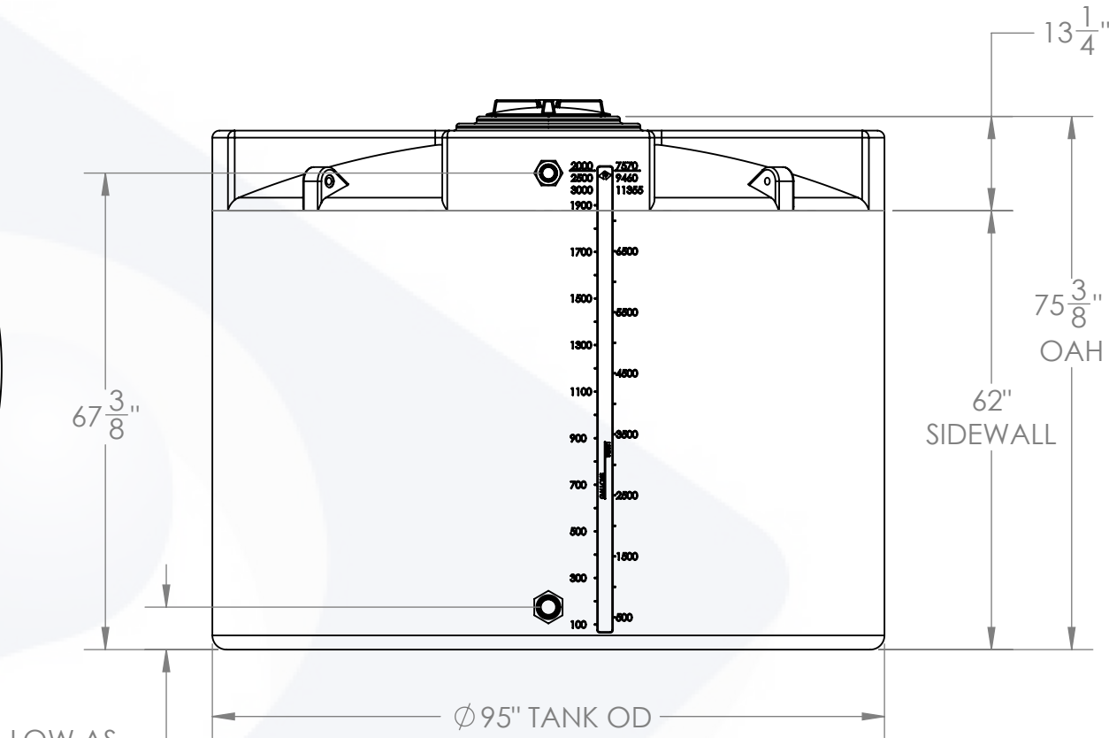
FRONT VIEW
