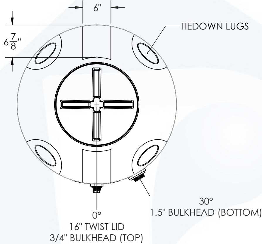
PLAN VIEW
