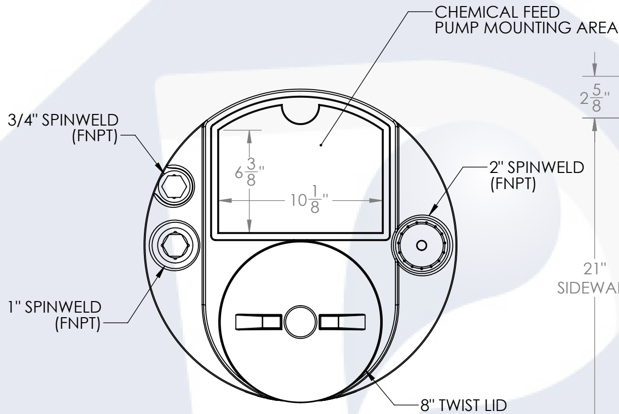
PLAN VIEW
