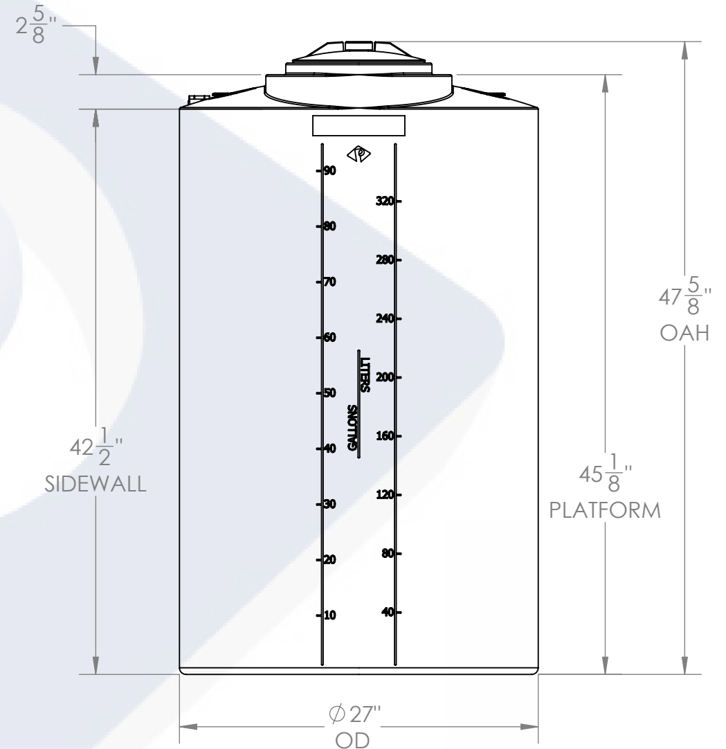
FRONT VIEW
